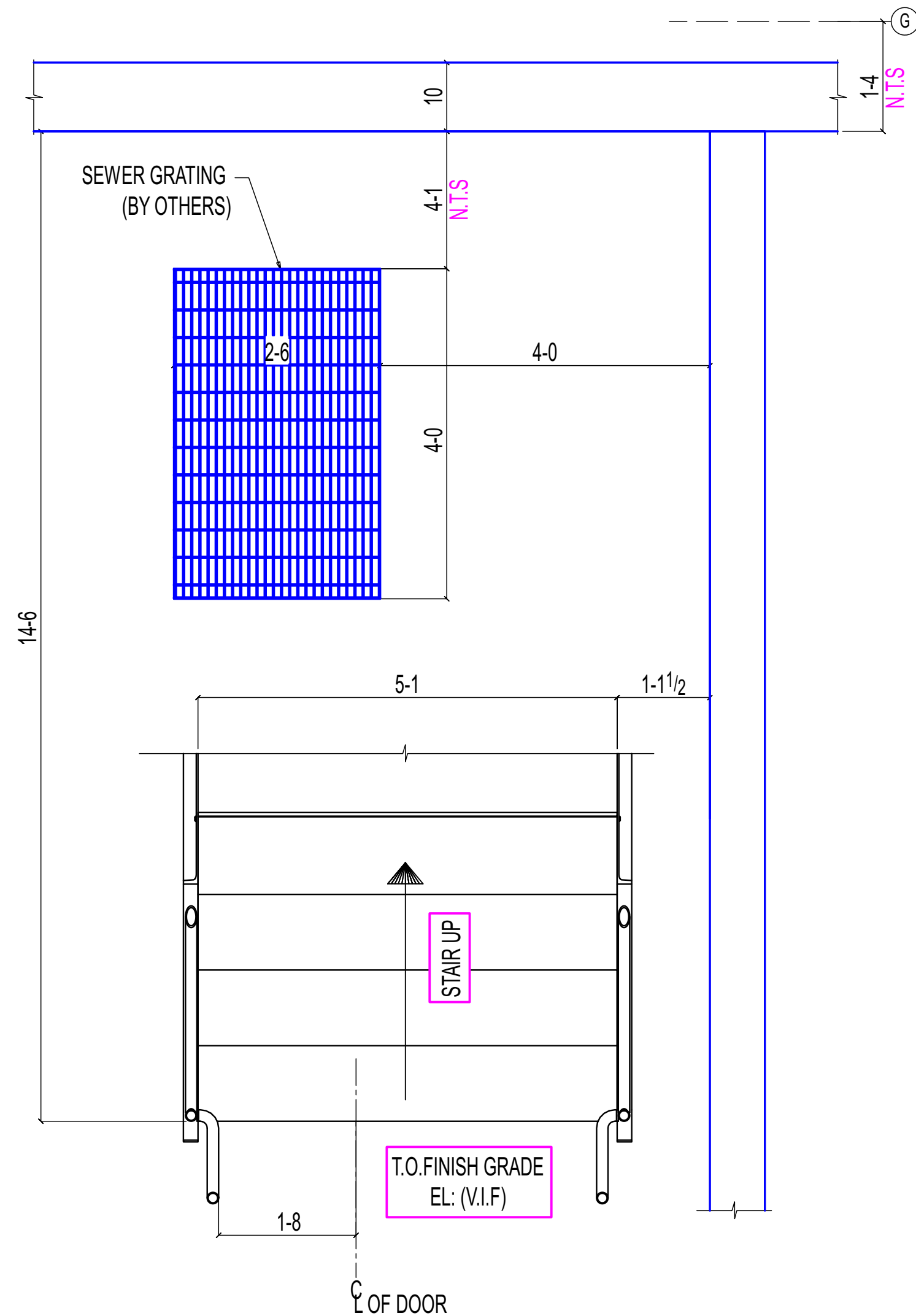
2 DOCK STAIR PARTIAL FRAMING PLAN (REF: 1/A101,14/A380) OTHERS NOT SHOWN FOR CLARITY
